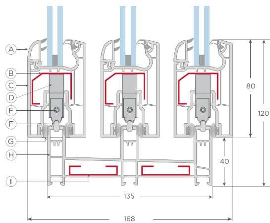
CORTE VENTANA NEW S75/80 TRIPLE RIEL
